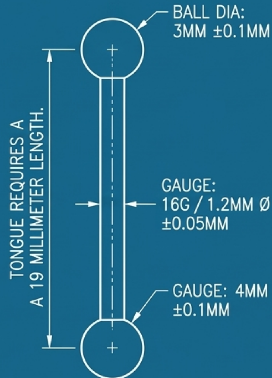
STRAIGHT BARBELL
